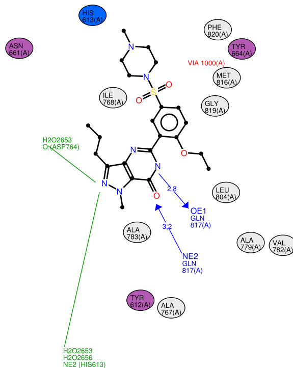
Figure 4 Example of user-customised diagram produced by LeView. Figure 4 shows an example of diagram generated by LeView for the PDE5 inhibitor sildenafil (PDB entry 1UDT [8]) after user customisation. The ligand appears in black. Hydrogen bonds are represented by blue arrows from donor to acceptor and the distance is displayed. Nearby residues are represented by ovals coloured depending on charge properties (non-polar residues in grey, acidic residues in red, basic residues in blue and uncharged polar residues in purple). Two water-mediated hydrogen bonds appear in green. The number of water molecules is indicated by the number of H2O.
