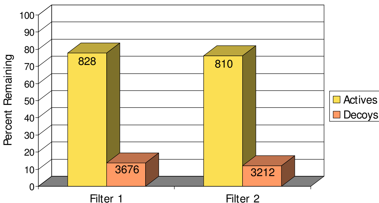
Figure 6 Bar chart illustrating filtering rates for actives vs. decoys with CDK2. The percentages of actives (true positives) and decoys (false positives) that remain in the docked database after each of the pharmacophore filters. The absolute number in each group of compounds is marked at the top of the bars.
