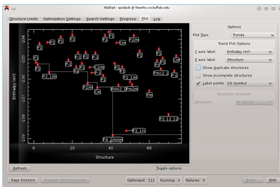
Figure 14 The XtalOpt extension. XtalOpt extension showing a plot of stability vs. search progress for a TiO 2 supercell.
