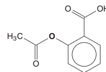
Figure 5 Structure of aspirin, composed from two sub-molecules. This hand-written example illustrates the use of chemfig's submol mechanism. Two named sub-molecules are defined, which can then be referenced to compose the complete molecule.
