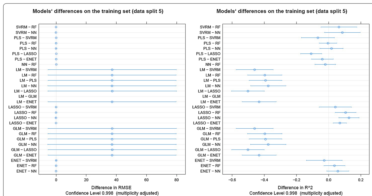
Fig. 6 Models' differences for protein corona training set (data split 5). Differences for R 2 and RMSE values among the applied models are presented. The average performance with two-sided confidence limits are plotted as derived by the Student t-test with Bonferroni multiplicity correction. We can observe that LM and GLM models are not fitting the data very well (large RMSE values)
